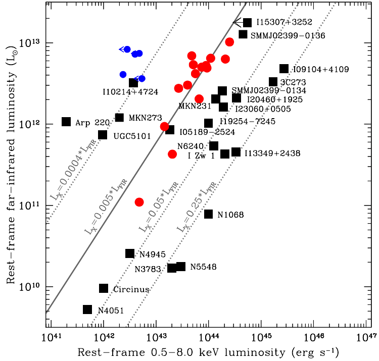
Figure 9: Far-infrared luminosity versus absorption-corrected X-ray luminosity for submillimeter galaxies in the CDF-N. Red filled circles indicate submillimeter galaxies believed to contain AGN, whereas smaller blue filled circles indicate submillimeter galaxies that are plausibly pure starbursts. Labeled black squares denote well-known AGN-dominated and star-formation dominated sources from the literature as well as two distant well-studied submillimeter galaxies containing AGN (SMM 02399–0134 and SMM 02399–0136). Slanted lines show ratios of constant X-ray to far-infrared luminosity. This ratio is typically \approx 3\text{--}30\% for AGN-dominated sources; many of the CDF-N submillimeter sources appear to contain moderate-luminosity AGN, but these AGN are unlikely to dominate the bolometric luminosity. Adapted from Alexander et al. (2005).
