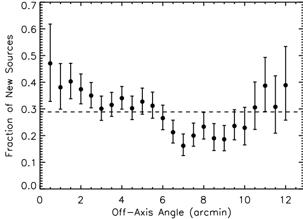
Figure 21. Fraction of new sources as a function of off-axis angle in arcmin bins of 1' , excluding the three new sources outside the 4 Ms CDF-S footprint. The error bars are the 1\sigma Poisson uncertainties (Gehrels 1986). The horizontal dashed line represents the total fraction of new sources ( 291/1008 = 29\% ). The rise of the new-source fraction beyond an off-axis angle of \approx 10' is likely caused by the dominating population of new sources detected in the more sensitive 2–7 keV band adopted in the 7 Ms CDF-S rather than the 2–8 keV band in the 4 Ms CDF-S.
