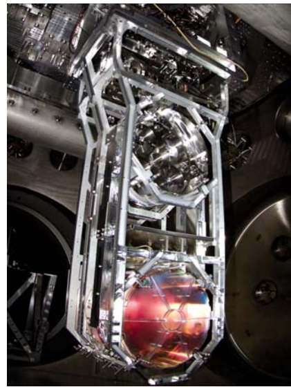
FIGURE 3. EACH MIRROR in LIGO's optical cavities sits at the end of a so-called quadruple pendulum. The 40 kg mirror (bottom) is not attached to the outside frame but hangs from the 40 kg silica cylinder above it by a set of fused silica fibers. The cylinder in turn hangs from a metal mass, which is hanging from yet another suspended metal mass. The system is designed to minimize thermal noise and passively dampen any environmental vibrations that get past LIGO's active seismic isolation system. (Courtesy of Caltech/MIT/LIGO Laboratory.)
