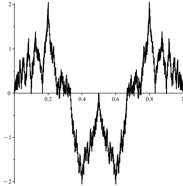
Figure 17.1 Graph of \text{Re } g(x) with g defined as in (E:Def f, g) (I7.35).
