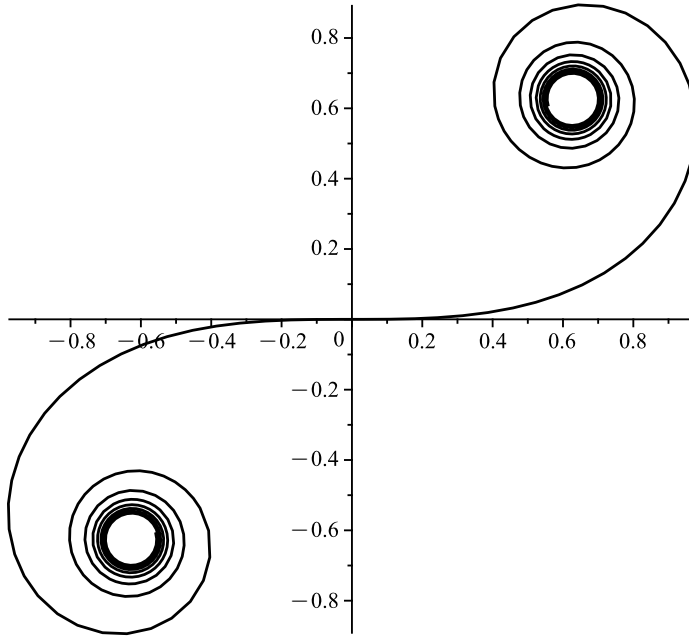
Figure 16.1 Graph of z(t) = \int_0^t e^{iu^2} du for -7 \leq t \leq 7 .
