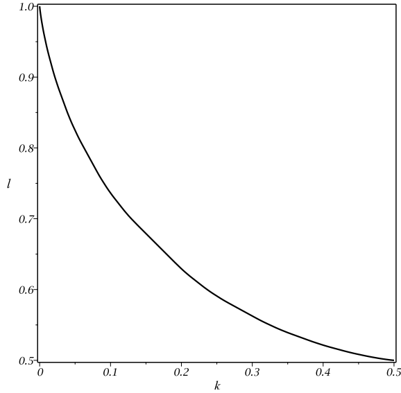
Figure 16.3 Polygonal path determined by 386 exponent pairs.
